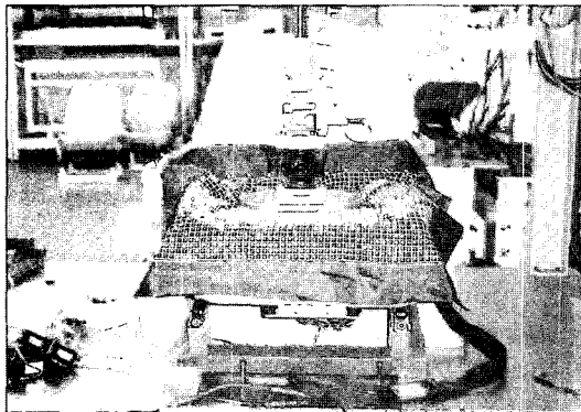
Figure 2. X-sensor system to measure pressure distribution.
