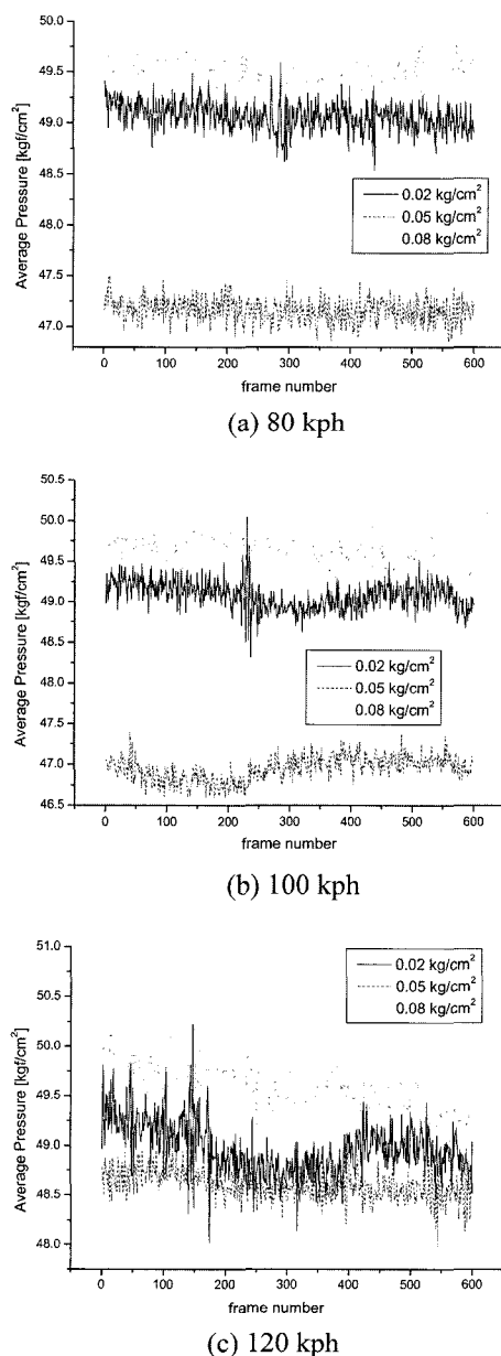
Figure 8. Measurement of average pressure depending on the vehicle speed (in case of 65 kg person).
