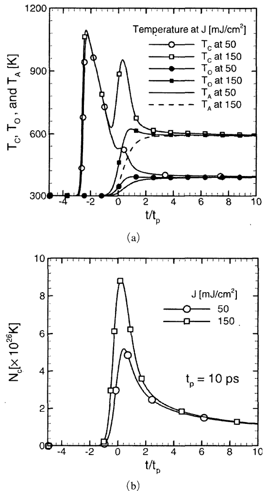
Fig. 4 Time evolutions of (a) carrier, LO phonon, acoustic phonon temperatures, and (b) carrier number densities for different fluences at t_p=10 \text{ ps}
