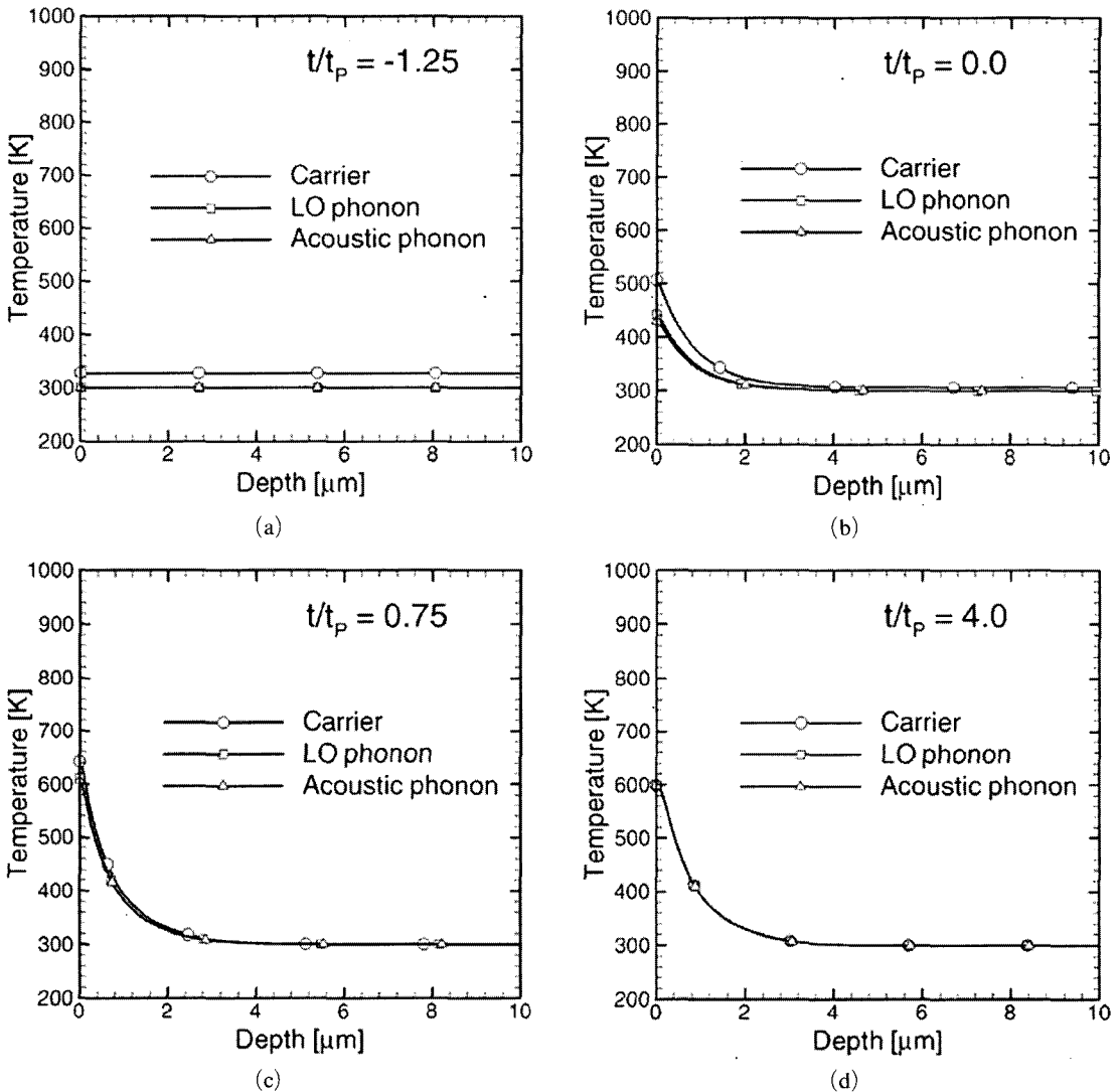
Fig. 7 Spatial temperature distributions of carriers, LO phonons, and acoustic phonons for 150 \text{ mJ/cm}^2 and t_p=200 \text{ ps} at different time locations
