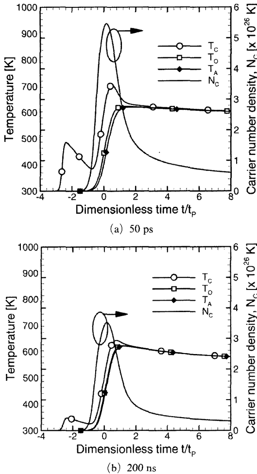
Fig. 5 In situ behaviors of carrier, LO phonon, acoustic phonon temperatures, and carrier number densities for 150 mJ/cm 2 at different pulse durations
