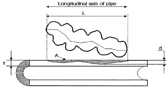
Fig. 1 A simplification of a corroded surface flaw in a pipeline
