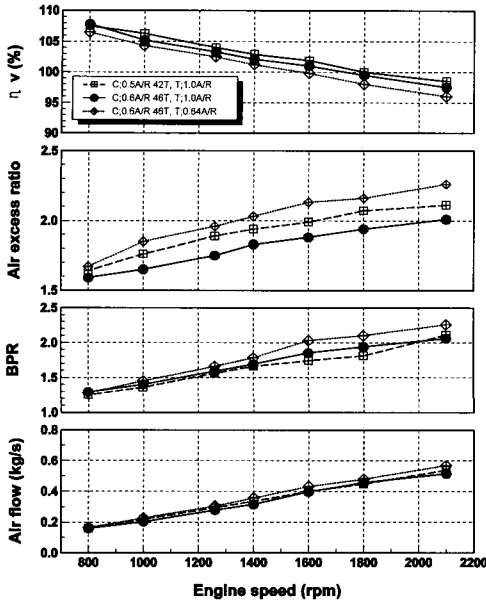
Fig. 10 Intake flow characteristics for three types of turbochargers
