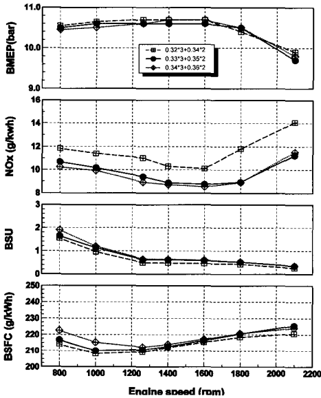
Fig. 4 Full load performance curves for three types of nozzle hole diameter
