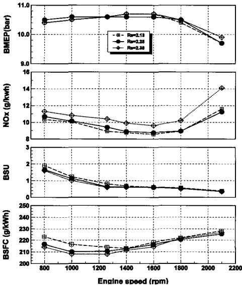
Fig. 3 Full load performance curves for three types of swirl ratio
