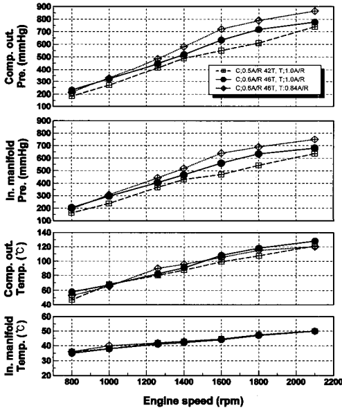
Fig. 11 Intake pressure and temperature change for three types of turbochargers
