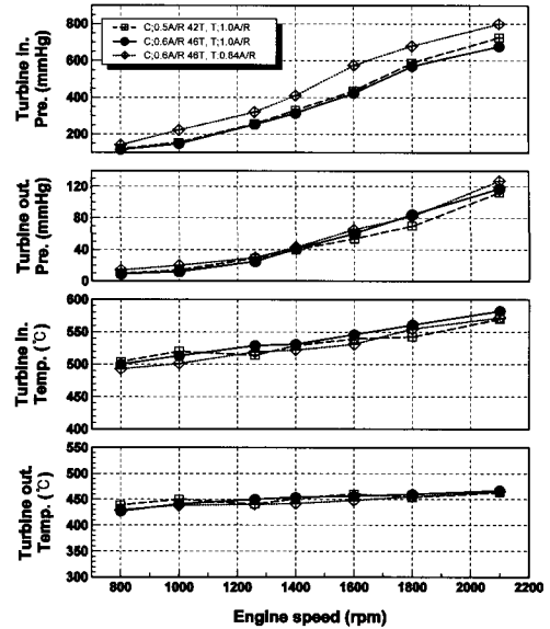
Fig. 12 Exhaust pressure and temperature change for three types of turbochargers
