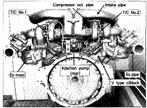
Fig. 1 Assembly of V8 type TCI diesel engine
