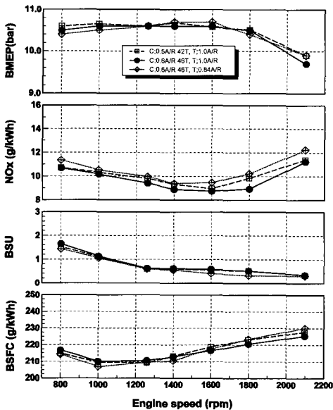
Fig. 9 Full load performance curves for three types of turbochargers
