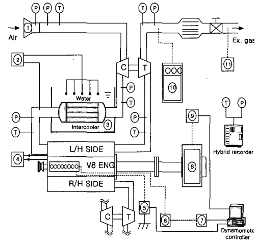
Fig. 1 Assembly of V8 type TCI diesel engine
