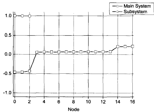
(a) 1st mode shape
