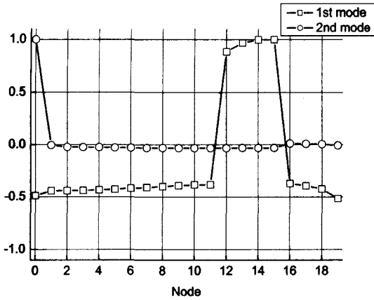
Fig. 11 Natural modes of computational model II with D-type coupling
