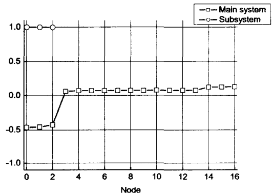
(a) 1st mode shape
