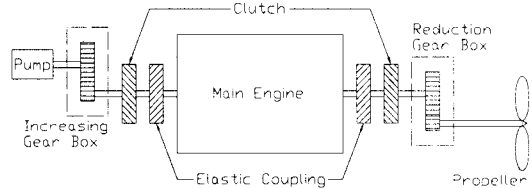
Fig. 1 Schematic diagram of engine shafting driving propeller and hydraulic pump
