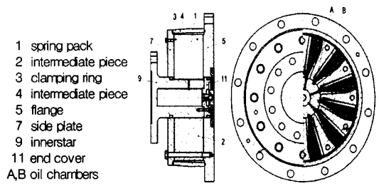
Fig. 2 The structure of the G-type coupling
