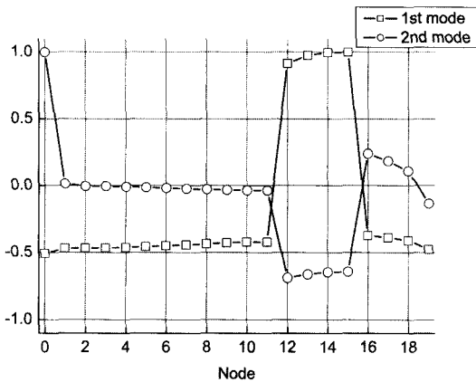
Fig. 8 Natural modes of model II with G-type coupling
