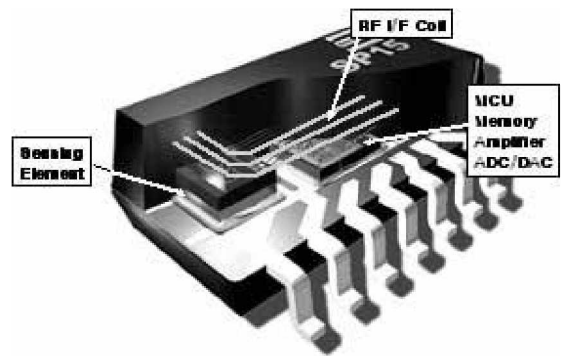
Smart Sensor With Wireless Interface
