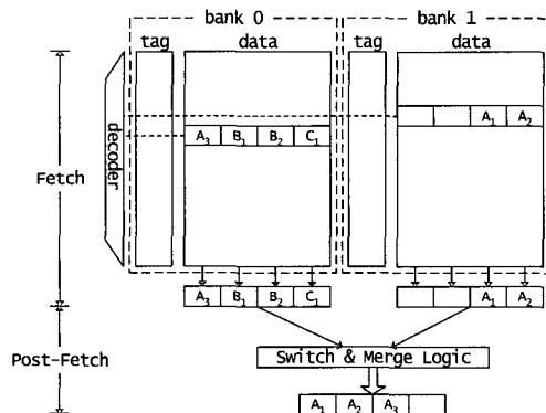
(Figure 1) The organization of the bank cache
