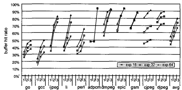
(b) 64-byte cache block (Figure 5) Buffer hit ratio
