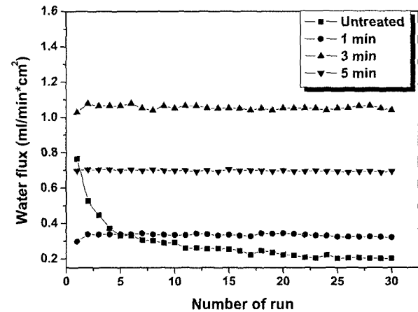
Figure 7. Water flux of untreated and AA plasma treated (70 mtorr, 20 W) membranes as a function of repeated number of filtration for various treatment times.
