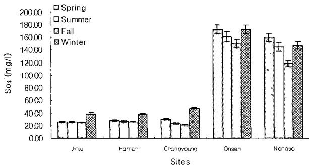
Fig. 10. Changes of SO 4 2- of throughfall collected at survey areas.
