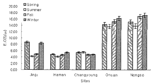
Fig. 3. Changes of EC of rainfall collected at survey areas.
