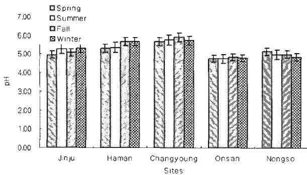
Fig. 1. Changes of pH by collection of rainfall at survey areas.
