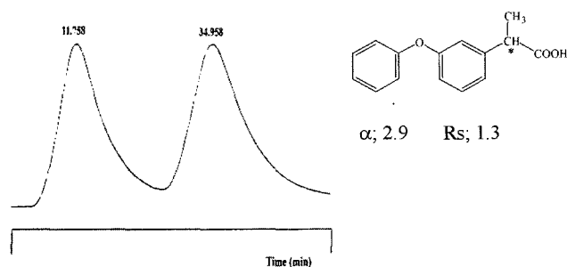
Fig. 3. Separation of fenoprofen racemates by HPLC with Cys-bonded chiral phases.
