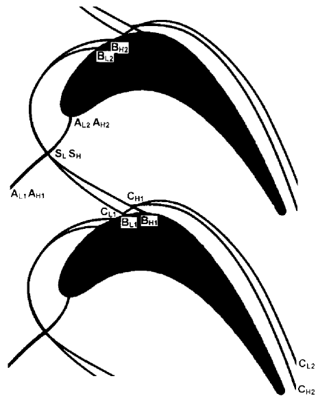
Fig. 9 Comparison of endwall flow boundaries between the low and high turbulence cases
