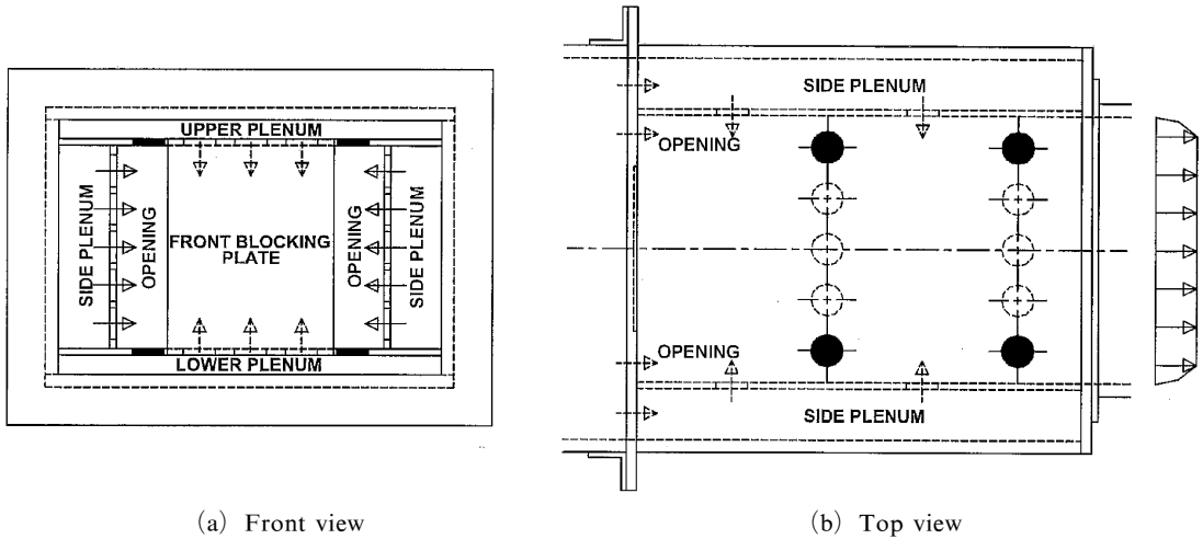
Fig. 3 Detail of high turbulence generator
