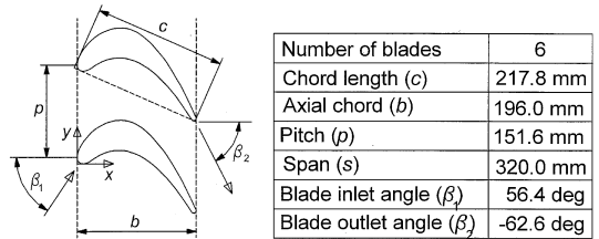
Fig. 2 Arrangement of turbine blade cascade
