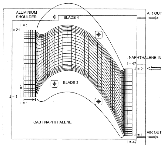
Fig. 4 Measurement locations on the naphthalene-cast endwall
