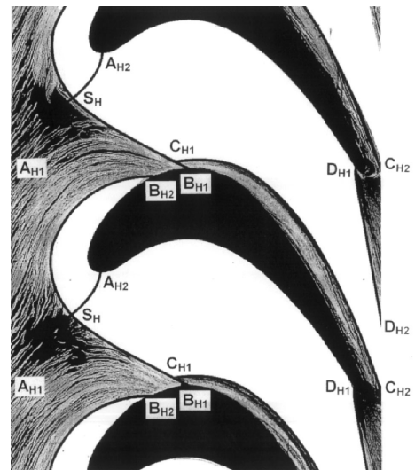
Fig. 7 Endwall surface flow visualization in Method 1 in the high turbulence case
