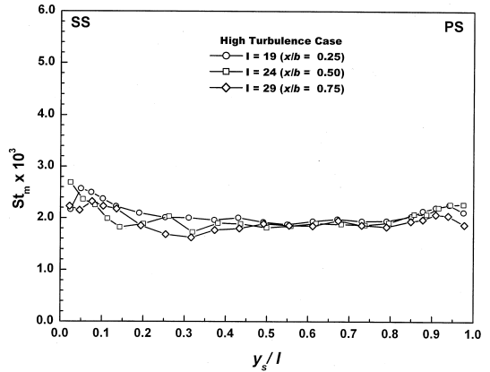
Fig. 15 Profiles of St_m along constant I lines in the high turbulence case
