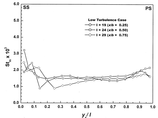
Fig. 12 Profiles of St_m along constant I lines in the low turbulence case
