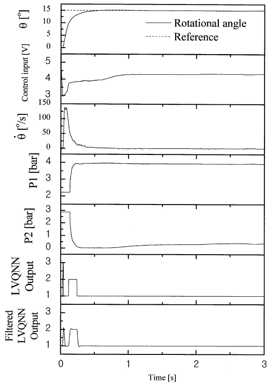
Fig. 13 Experimental results with no external inertia load (class 1)
