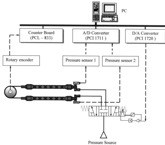
Fig. 1 Schematic diagram of the pneumatic artificial muscle manipulator
