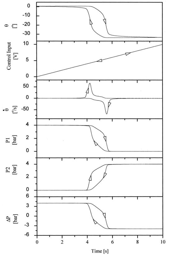
Fig. 5 Characteristics of the pneumatic artificial muscle manipulator
