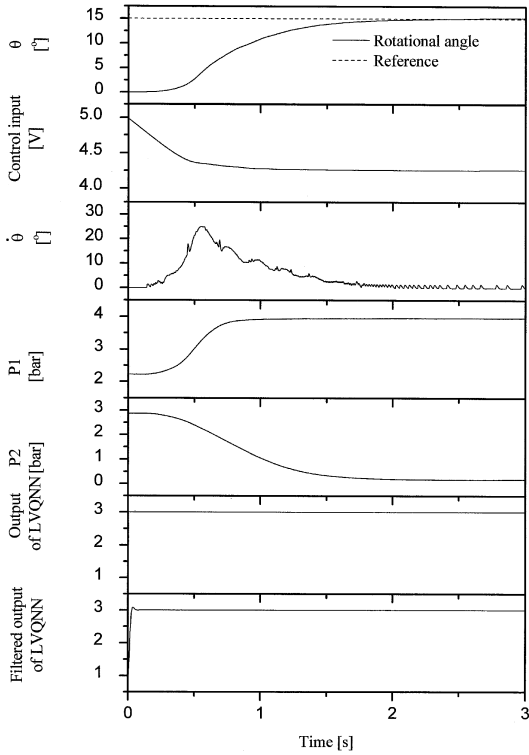
Fig. 15 Experimental results when external inertia load is 56.25[\text{g}\cdot\text{m}^2] (class 3)
