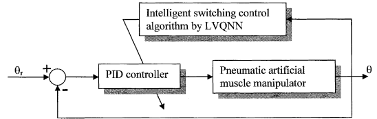
Fig. 7 Structure of the newly-proposed control algorithm
