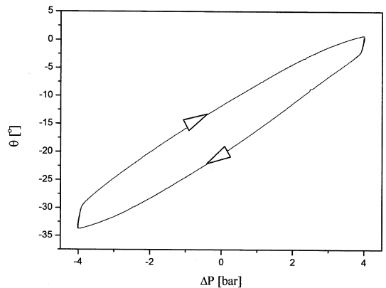
Fig. 6 Hysteresis of the pneumatic artificial muscle manipulator
