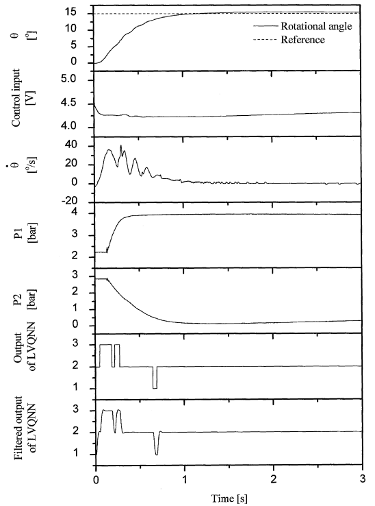
Fig. 14 Experimental results when external inertia load is 28.12 [g \cdot cm^2] (class 2)
