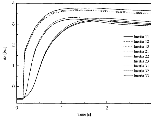
(e) Pressure Difference
