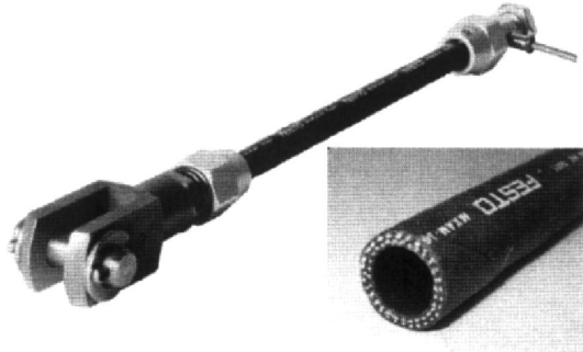
Fig. 2 Structure of the pneumatic artificial muscle
