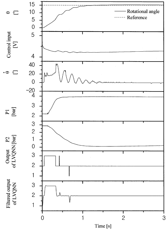
Fig. 16 Experimental results when external inertia load is 42.19[\text{g}\cdot\text{m}^2] (class 2 and class 3)
