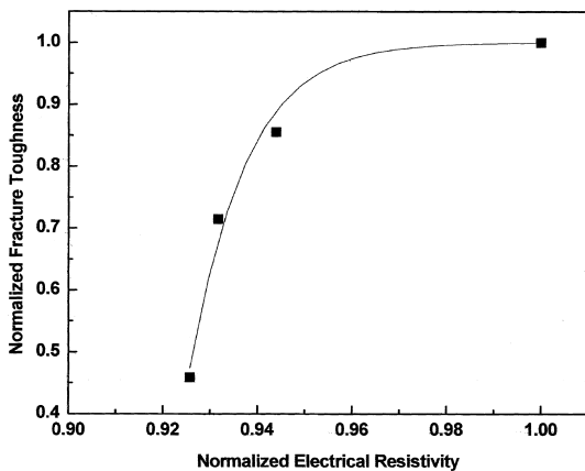
Fig. 7 Relation between normalized fracture toughness and normalized electrical resistivity
