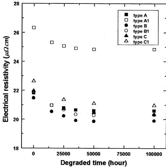
Fig. 3 Effect of degraded time on electrical resistivity
