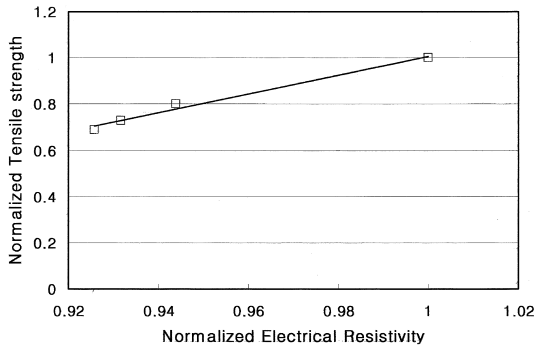
Fig. 6 Relation between normalized tensile strength and normalized electrical resistivity
