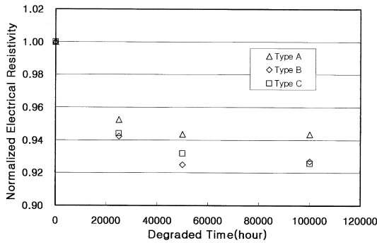
Fig. 4 Effect of normalized electrical resistivity on degraded time for different specimen type
