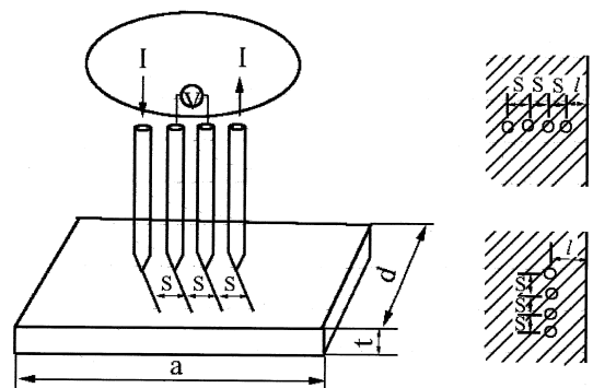
Fig. 1 Configuration of specimen boundary and 4 point probe
