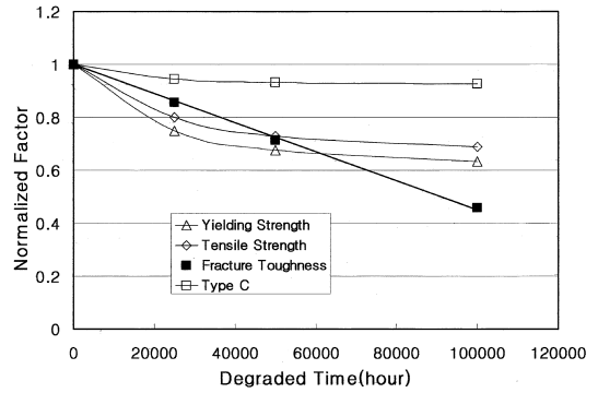
Fig. 5 Effect of normalized factors on degraded time
