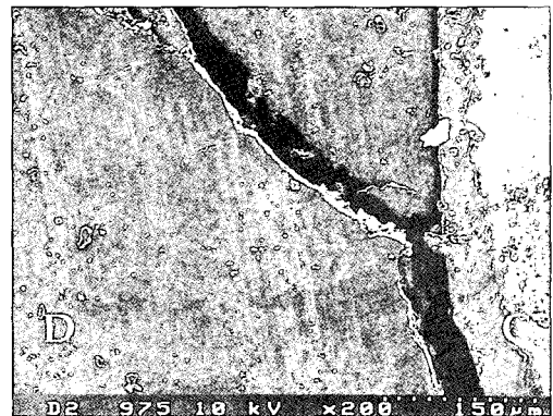
Fig. 10. The fractural interface of metal cast post and dentin (×200) (D : Dentin, C : Cast post)
