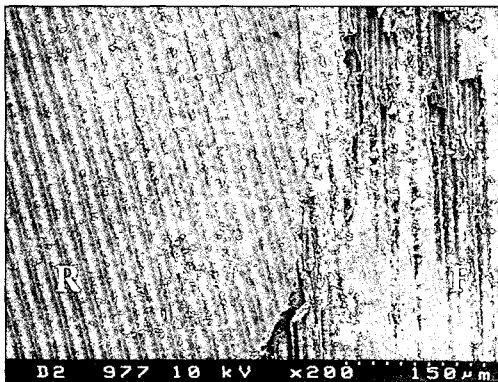
Fig. 9. The interface of glass fiber post and resin core in type C fracture(×200) (F : Glass fiber post, R : Resin core)
