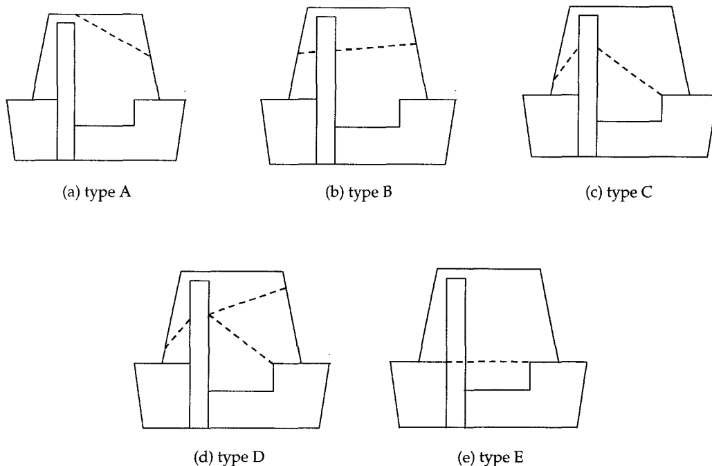
Fig. 2. Schematic representation of main fracture lines in catastrophic failure.
