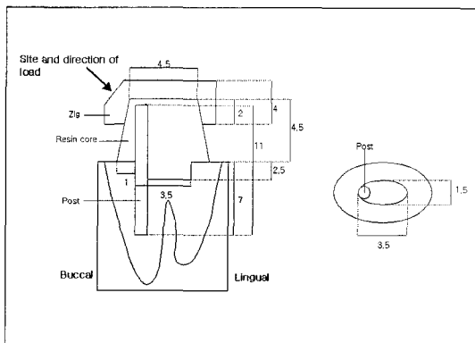
Fig. 1. Schematic drawing of test specimen showing dimensions in mm.
