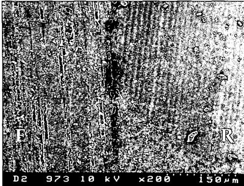
Fig. 5. The interface of glass fiber post and resin core in type A fracture(×200) (F : Glass fiber post, R : Resin core)
