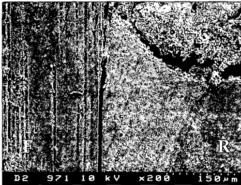
Fig. 7. The interface of glass fiber post and resin core in type B fracture(×200) (F : Glass fiber post, R : Resin core)
