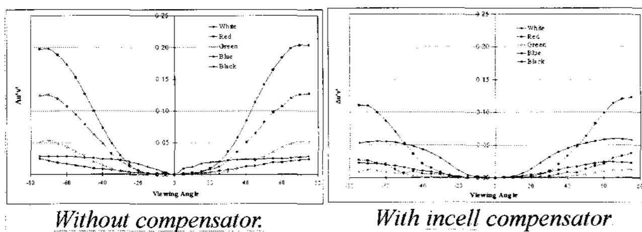
Fig. 8. \Delta u'v' plots in the 45^\circ diagonal direction for the PVA panels with and without an incell biaxial RM compensator.
