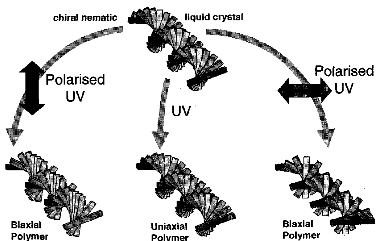
Fig. 3. Diagram showing how different forms of UV light can be used to change the optical properties of a tight pitch, cholesteric RM film. The direction of plane polarised light defines the slow axis of the biaxial film.
