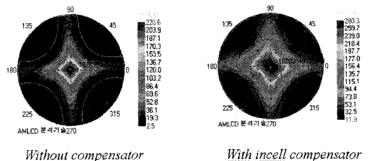
Fig. 6. Isocontrast plots of the prototype with and without incell RM biaxial compensator.
