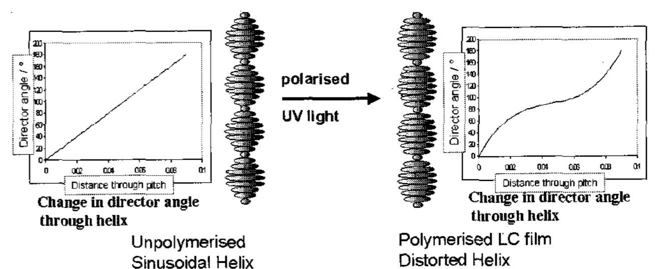
Fig. 2. Schematic representation of the potential structure of the helix in the uniaxial and biaxial films.
