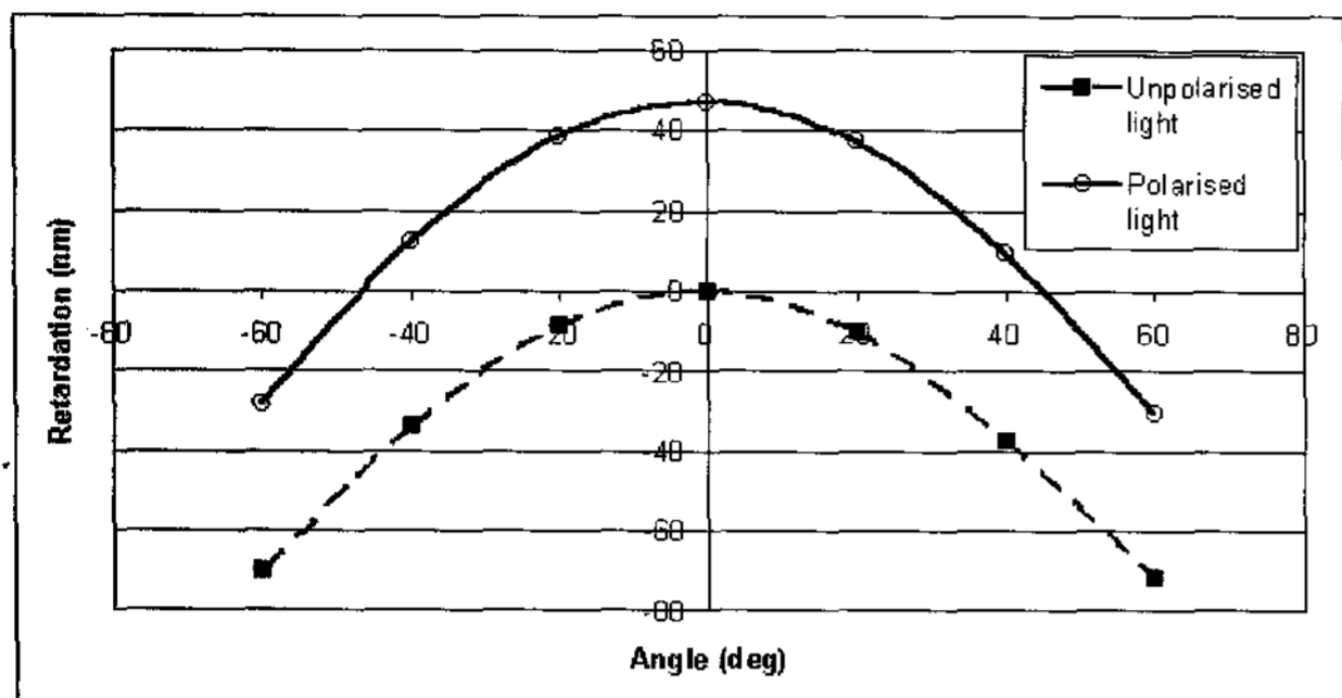
Fig. 4. Retardation profile of an Uniaxial and a biaxial tight pitch cholesteric RM film.
