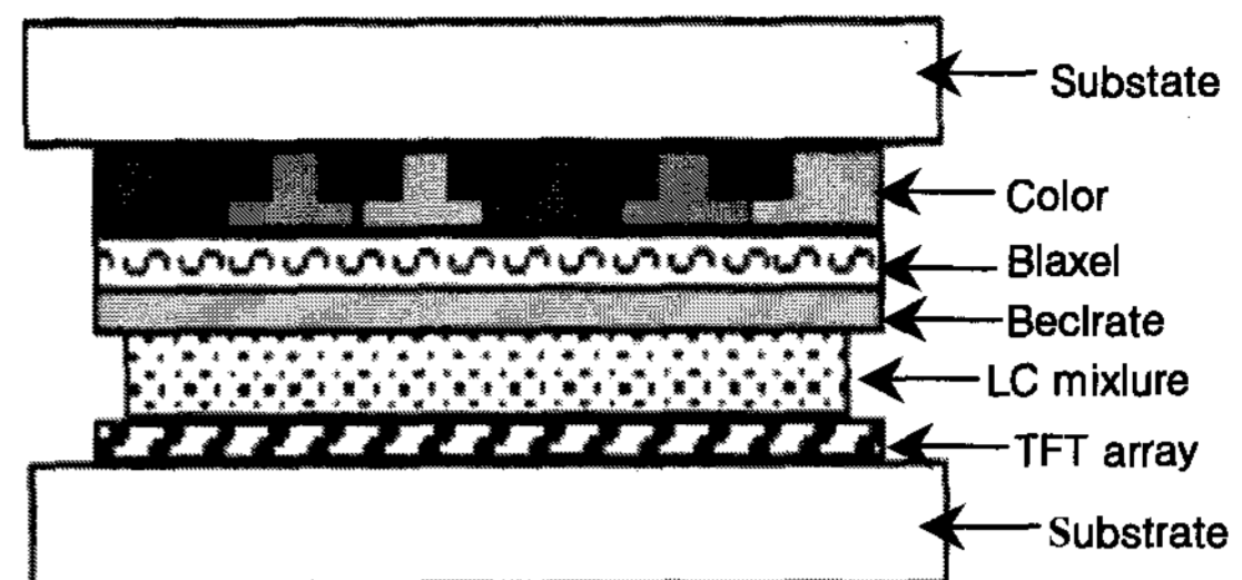
Fig. 5. Schematic representation of the prototype PVA cell containing an incell RM biaxial retarder film.
