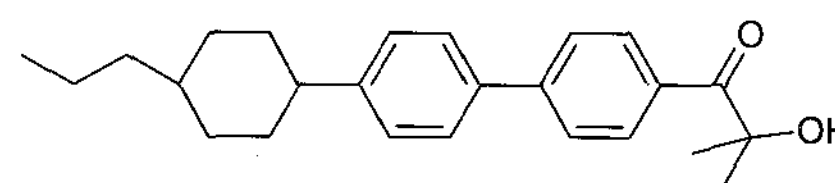
Fig. 1. The structure of a dichroic photoinitiator used to make biaxial RM films.
