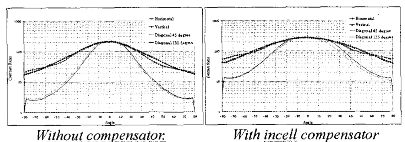
Fig. 7. Contrast ratio against incident angle for a PVA panel with and without an incell biaxial RM compensator.
