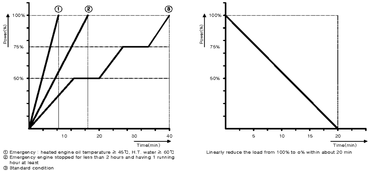
Fig. 1 Loading & unloading process
