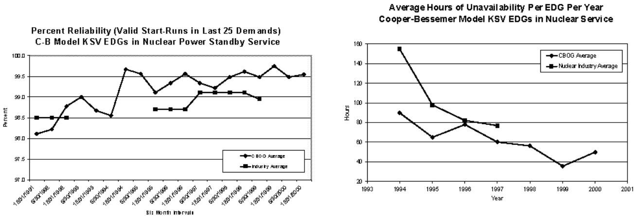
Fig. 2 Reliability of EDGs in US
