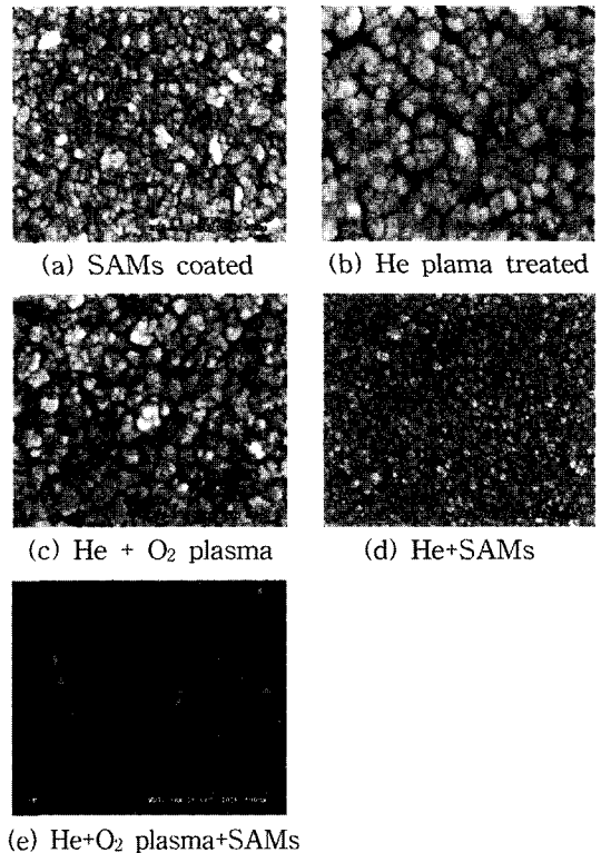
Fig. 3. The surface morphology of Cu coating layer treated each pretreatment conditions.
