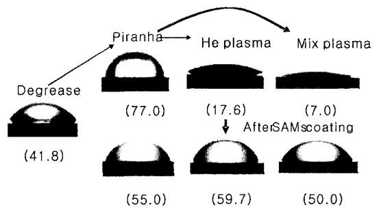
Fig. 1. The change of contact angle.
