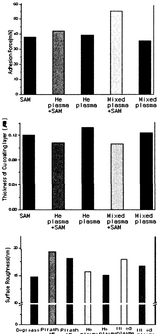
Fig. 2. Results of nano indenter scratch test. (Thickness of coating layer)
