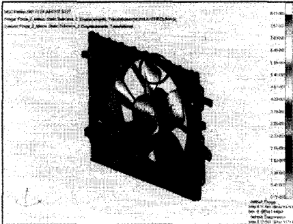
Fig. 12 Maximum displacement of CFA(Z-axis direction load)
