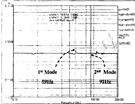
Fig. 16 CFA vibration test result(1 st , 2 nd mode)
