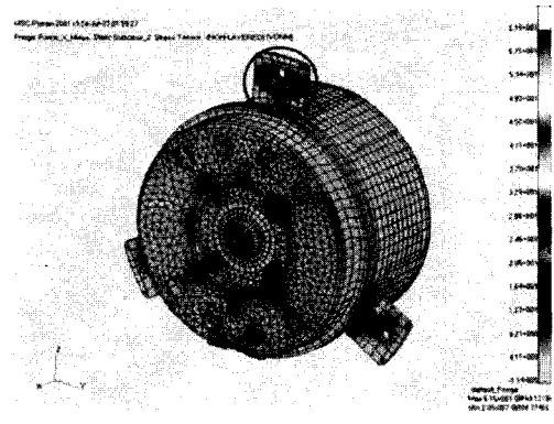
Fig. 11 Maximum stress of DC motor(X-axis direction load) : 62 MPa
