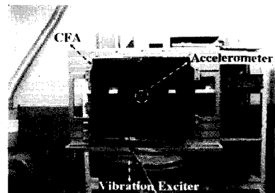
Fig. 15 CFA vibration test set
