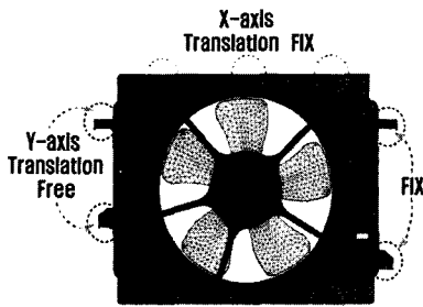
Fig. 8 Boundary condition of CFA for static analysis
