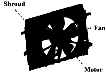
Fig. 1 3D CAD model of CFA
