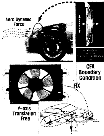
Fig. 5 Boundary condition of FE model for CFA
