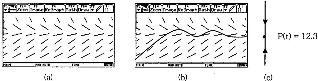
<Figure 1> Slope field for dP/dt = 0.6P(1 - P/12.3)
