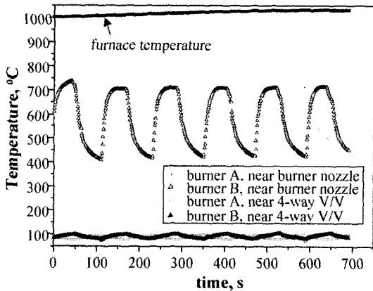
Fig. 4. Temperature histories of the regenerator (Fuel: LPG).
