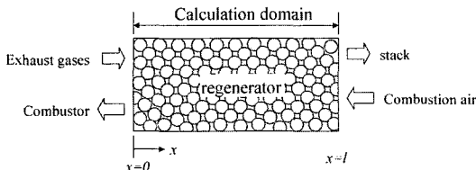
Fig. 1. Calculation domain of heat regenerator.
