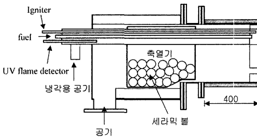
(a) Schematic diagram of the burner
