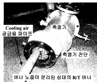
(b) photo of the burner
