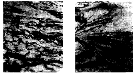
Fig. 5 Fracture surfaces ( \times 120 ) of resin castings obtained by flexural test: (a) DGEBF/EDA, (b) DGEBF/HMDA post-cured system.
