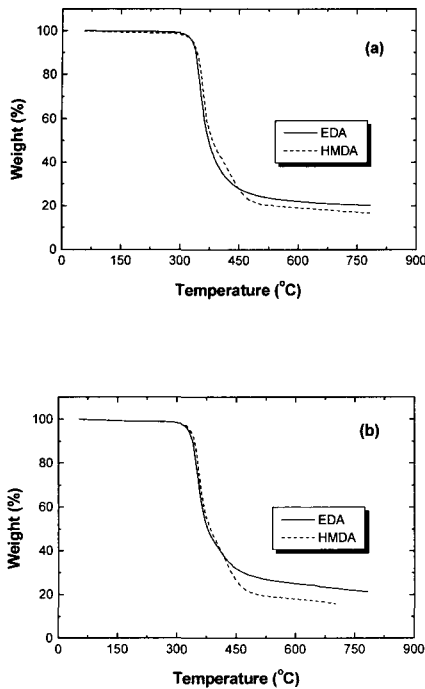
Fig. 3 TGA thermograms for the DGEBF/linear amine cure system: (a) preliminary-cured; (b) post-cured.
