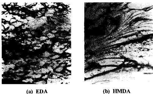
Fig. 4 Fracture surfaces ( \times 120 ) of resin castings obtained by flexural test: (a) DGEBF/EDA, (b) DGEBF/HMDA preliminary-cured system.
