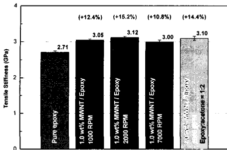
Fig. 6 Tensile stiffness with changes of the mixing ratio of epoxy resin and solvent and homogenizing speed.
