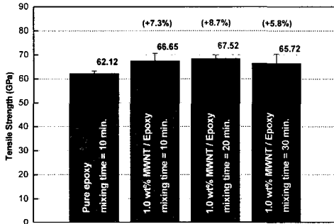
Fig. 14 Tensile strength according to mixing time of (MWNT + epoxy resin) and hardener.
