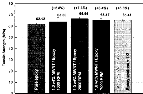
Fig. 7 Tensile strength with changes of the mixing ratio of epoxy resin and solvent and homogenizing speed.
