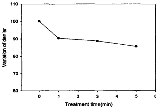
Fig. 2. Variation of denier with treatment time.
