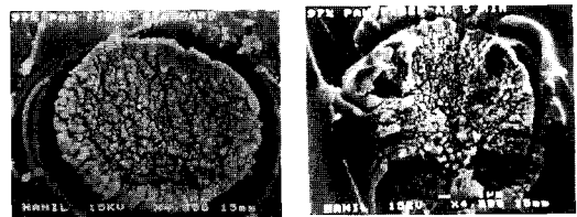
Fig. 6. Images of cross-section of polyacrylonitrile fiber; A: untreated fiber B: argon-plasma-treated fiber at 240 mTorr, 40 W for 5 min.
