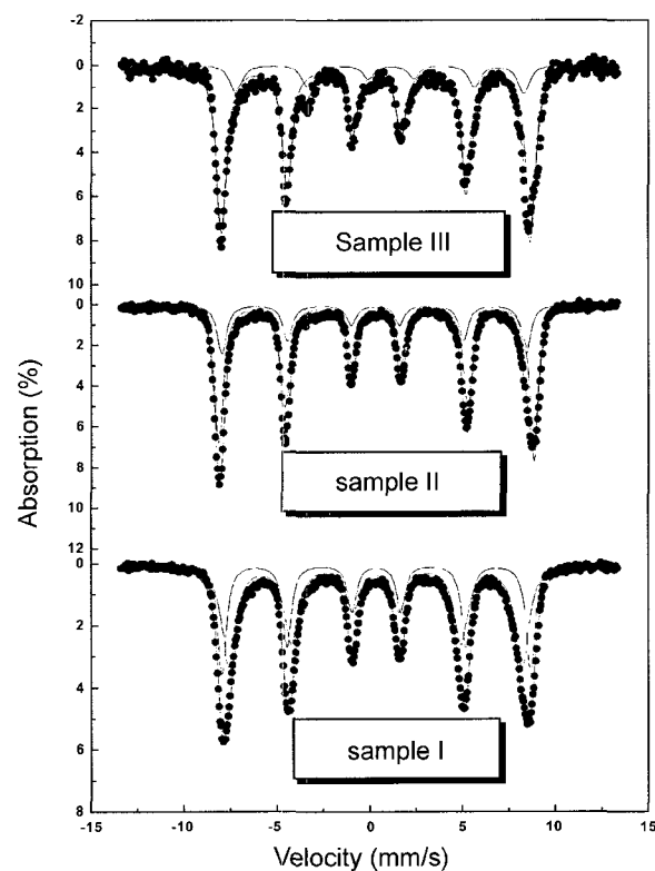
Fig. 3. The Mössbauer spectra of all of samples measured at 13 K.
