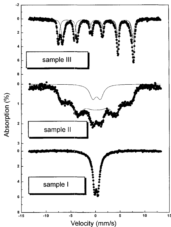
Fig. 2. The Mössbauer spectra of all of samples measured at room temperature.
