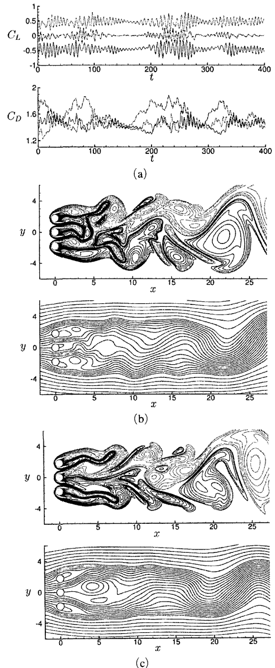
Fig. 4 Flip-flopping wake pattern behind three side-by-side cylinders: (a) time evolutions of the lift and drag coefficients, and (b) and (c) instantaneous vorticity contours and streamlines (respectively t=200 and 400 ) at g^*=0.8 and Re=100
