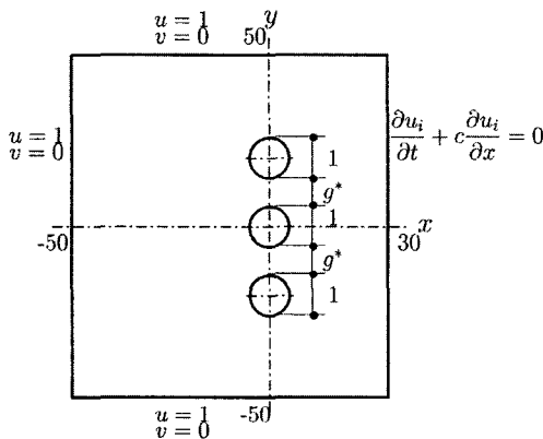
Fig. 1 Schematic diagram of the present computational domain
