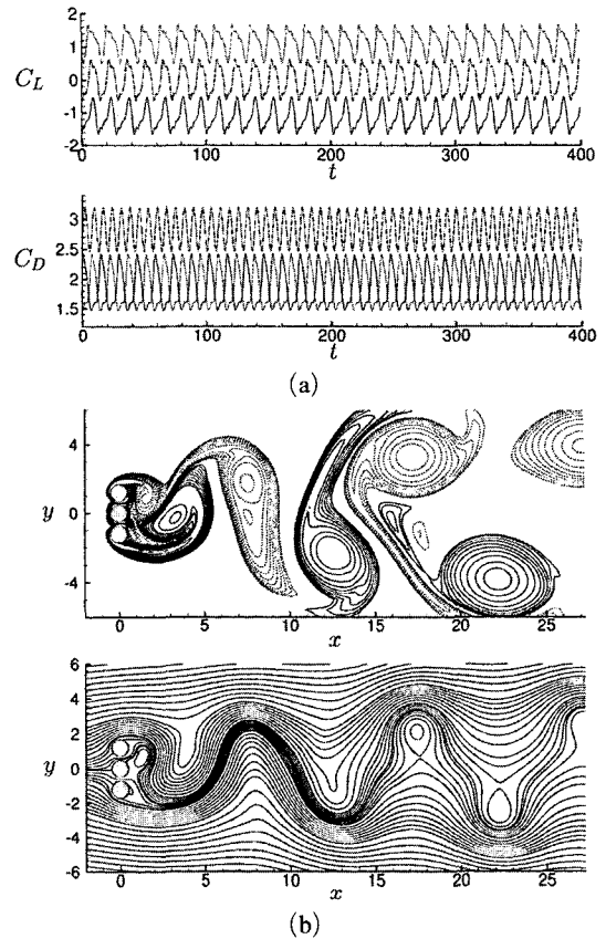
Fig. 7 Single bluff-body wake pattern behind three side-by-side cylinders: (a) time evolutions of the lift and drag coefficients, and (b) instantaneous vorticity contours and streamlines at g^*=0.2 and Re=100
