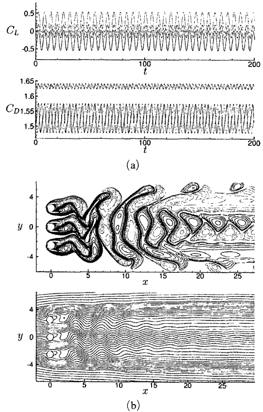
Fig. 3 Inphase-synchronized wake pattern behind three side-by-side cylinders: (a) time evolutions of the lift and drag coefficients, and (b) instantaneous vorticity contours and streamlines at g^*=1.5 and Re=100
