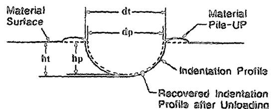
Fig. 2 Schematic diagram of a ball indentation profile
