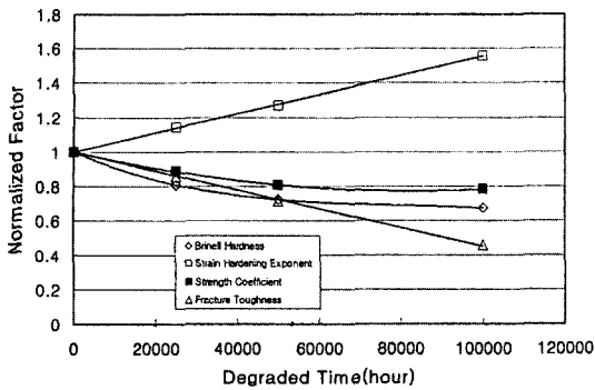
Fig. 6 Effect of normalized factor on equivalent degraded time at service temperature
