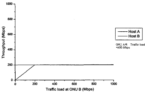
(b) 단말별 Throughput (Each Station's Throughput)
