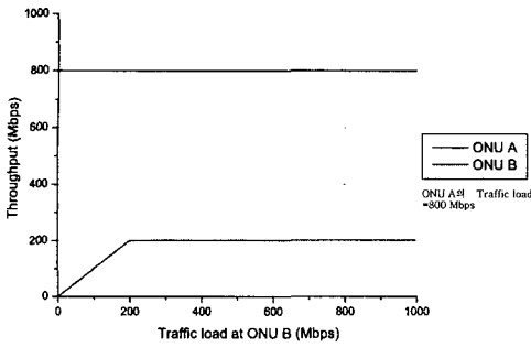
(a) ONU별 Throughput (Each ONU's Throughput)
