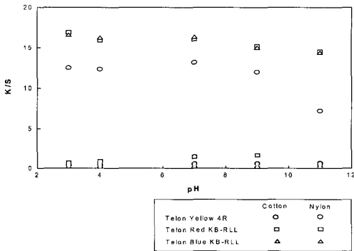
Fig. 8. The effect of pH on K/S value of cotton and nylon dyed with levelling type acid dyes.
