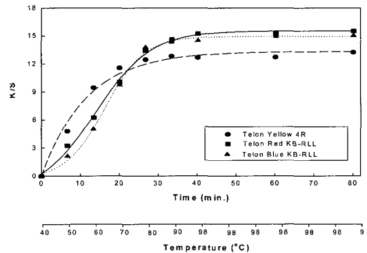
Fig. 5. The effect of temperature and time on K/S value of nylon dyed with levelling type acid dyes.
