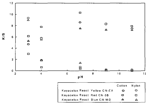
Fig. 7. The effect of pH on K/S value of cotton and nylon dyed with MNT type reactive dyes.
