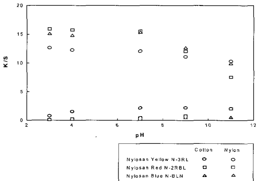
Fig. 9. The effect of pH on K/S value of cotton and nylon dyed with half-milling type acid dyes
