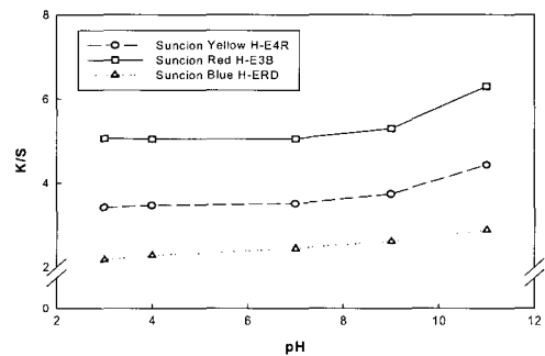
Fig. 2. The effect of pH on K/S value of cotton dyed with MCT type reactive dyes.
