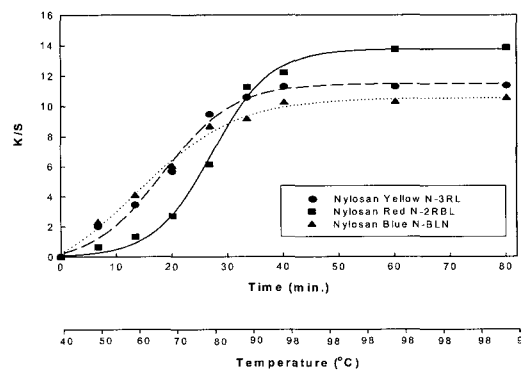
Fig. 6. The effect of temperature and time on K/S value of nylon dyed with half-milling type acid dyes.
