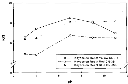
Fig. 1. The effect of pH on K/S value of cotton dyed with MNT type reactive dyes.
