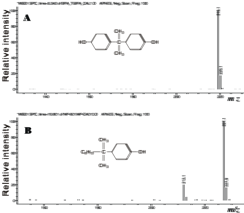
Fig. 4. ESI mass spectra of BPA (A) and NP (B) detected under negative conditions mode. Fragmentor, 100 V; standard concentration, 1 ppm; and injection volume, 30 \mu L for each compound in SCAN mode. Operation flow rate of BPA and NP were 0.2 mL/min and 0.4 mL/min, respectively.
