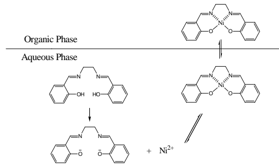
Fig. 3. Steps involved in solvent extraction of Ni(II) with salen.
