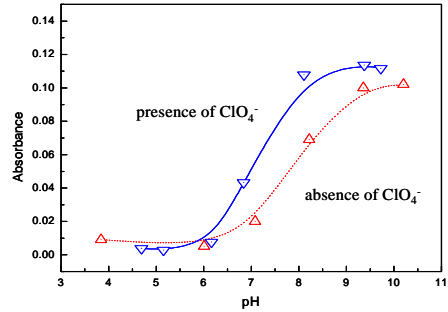
Fig. 7. Effect of equilibrated pH on extraction of Ni(II) in the presence of \text{ClO}_4^- ion or not.
