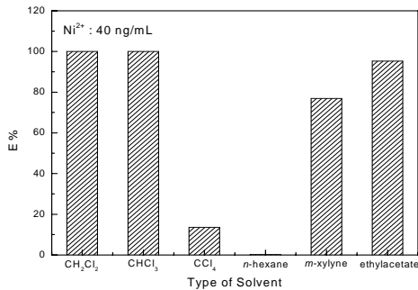
Fig. 4. Extraction efficiencies according to the type of solvent. Dielectric constants CH 2 Cl 2 :9.14, CHCl 3 : 4.807, CCl 4 :2.24, n -hexane:1.89, m -xylene:2.359, ethyl acetate:6.081.
