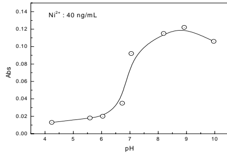
Fig. 5. Effect of equilibrated pH on the extraction of Ni(II).
