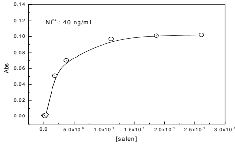
Fig. 6. Optimum concentration of salen for the formation of stable Ni-salen complex.
