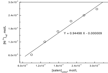
Fig. 2. Plot of extracted Ni(II) versus added salen.
