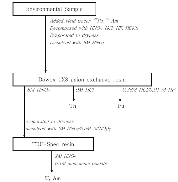
Fig. 1. Analytical procedure for the separation of actinides using extraction chromatography.
