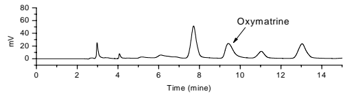
Fig. 8. Chromatogram of oxymatrine ; reflux extraction of Sophorae Radix 1 g in water at 80 °C for 3 hour.
