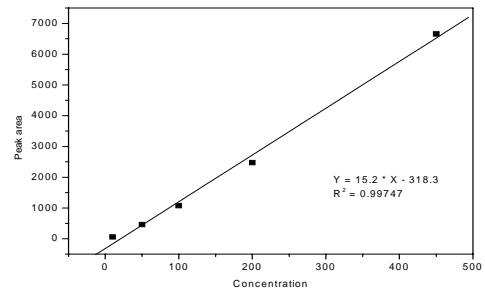
Fig. 2. Calibration curve of oxymatrine
