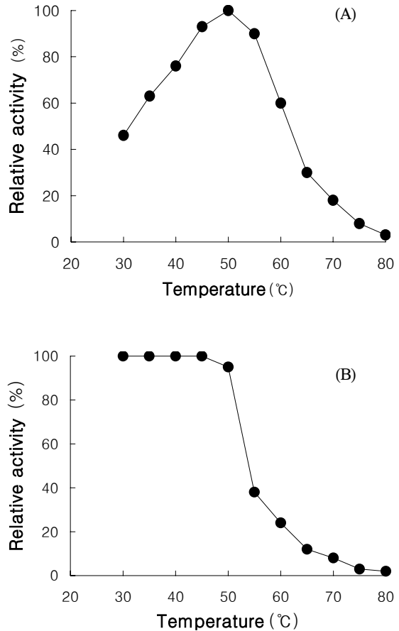
Fig. 4. Effects of temperature on the activity of the H. polymorpha alcohol oxidase. (A) Optimum temperature. In order to understand the effect of temperature, various temperature range, from 30 to 80 °C, of reaction mixture were investigated. (B) Heat stability. Thermal stability was determined by using the enzyme with a protein concentration of 0.1 mg/mL. Remaining alcohol oxidase activities were assayed after incubation for 10 min at each temperature.
