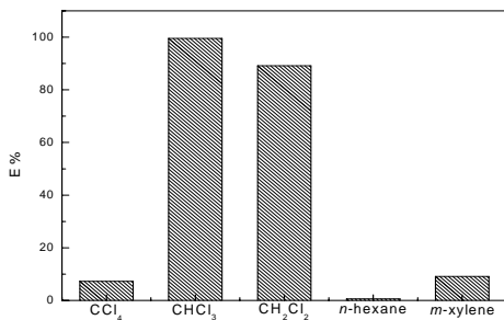
Fig. 1. Effect of solvent type on the extraction efficiency of Mn-complex from an aqueous solution at pH 5.
