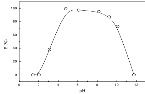
Fig. 2. Effect of solution pH on extraction efficiency of Mn(II).
