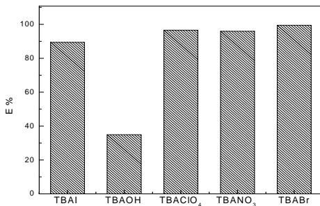
Fig. 3. Comparison of extraction efficiencies of Mn(II) according to the type of counter anion of tetrabutylammonium ion.
