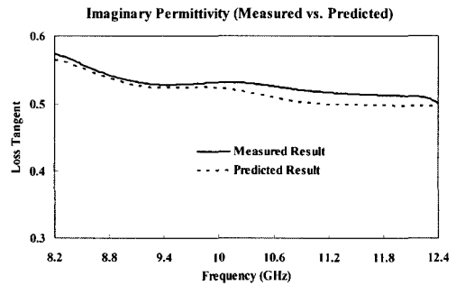
(b) imaginary part of the complex relative permittivity
