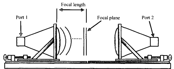
Fig. 4 Plane wave nature of electromagnetic fields in the spot-focusing horn lens antennas.
