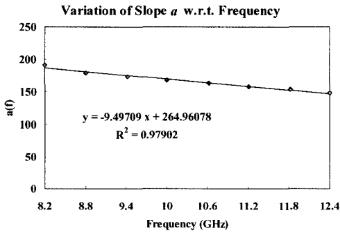
(a) slope a for the linear increment of the dielectric constant
