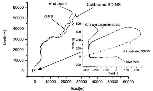
Fig. 3. The actual experiments of SDINS for calibration analysis 2.
