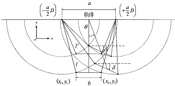
(b) The spreader inclination does not depend on rope lengths: RMQC.
