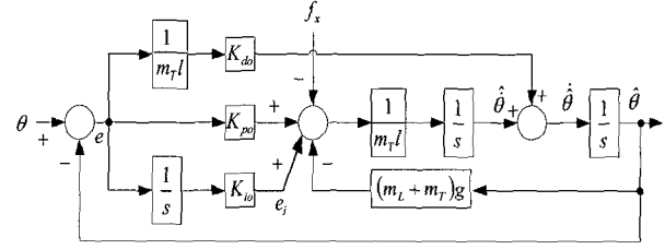
Fig. 4. Block diagram of the sway angular velocity observer.
