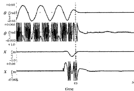
(b) l = 19.3 m, m_L = 17.2 ton (empty container).
