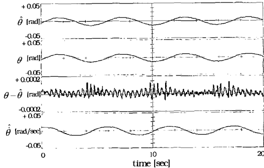
(a) For a free sway: \theta - \hat{\theta} is the error between measured and estimated angles.
