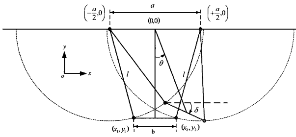
(a) RMQC (two-rope structure).
