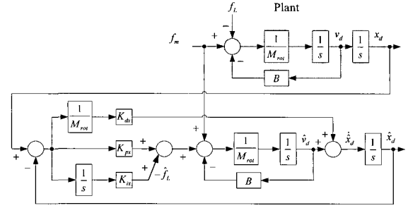
Fig. 5. Block diagram of the trolley velocity observer.
