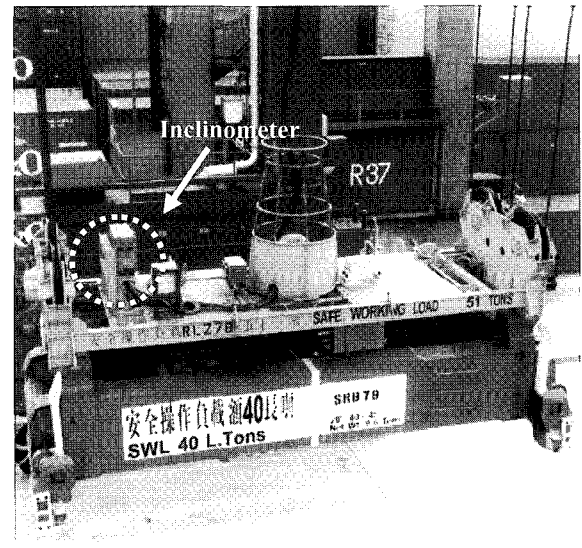
(b) The head block and an inclinometer.
