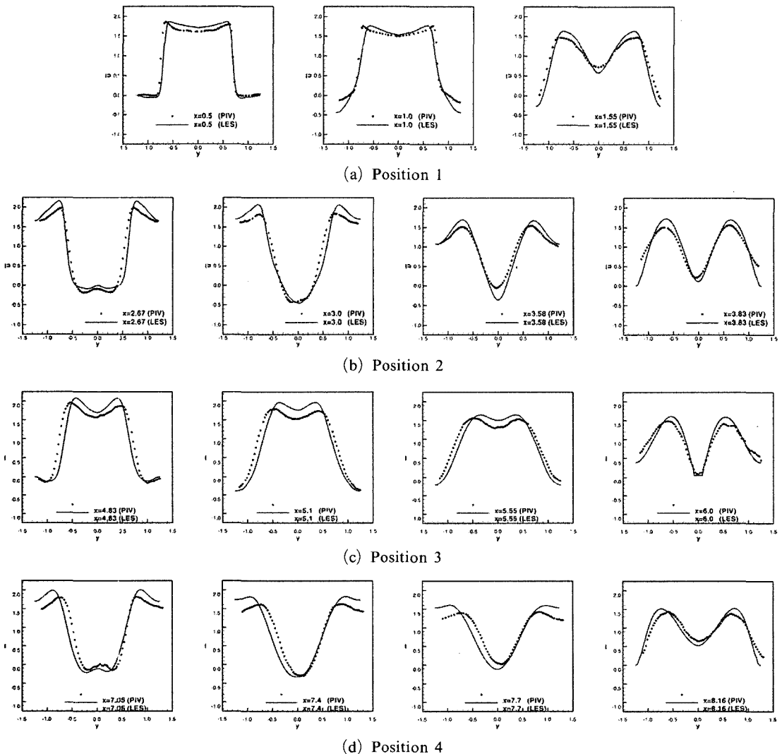
Fig. 6 Comparison of time-averaged streamwise velocity obtained from the present calculation with PIV experiment : (-) this study, (■) PIV experiment
