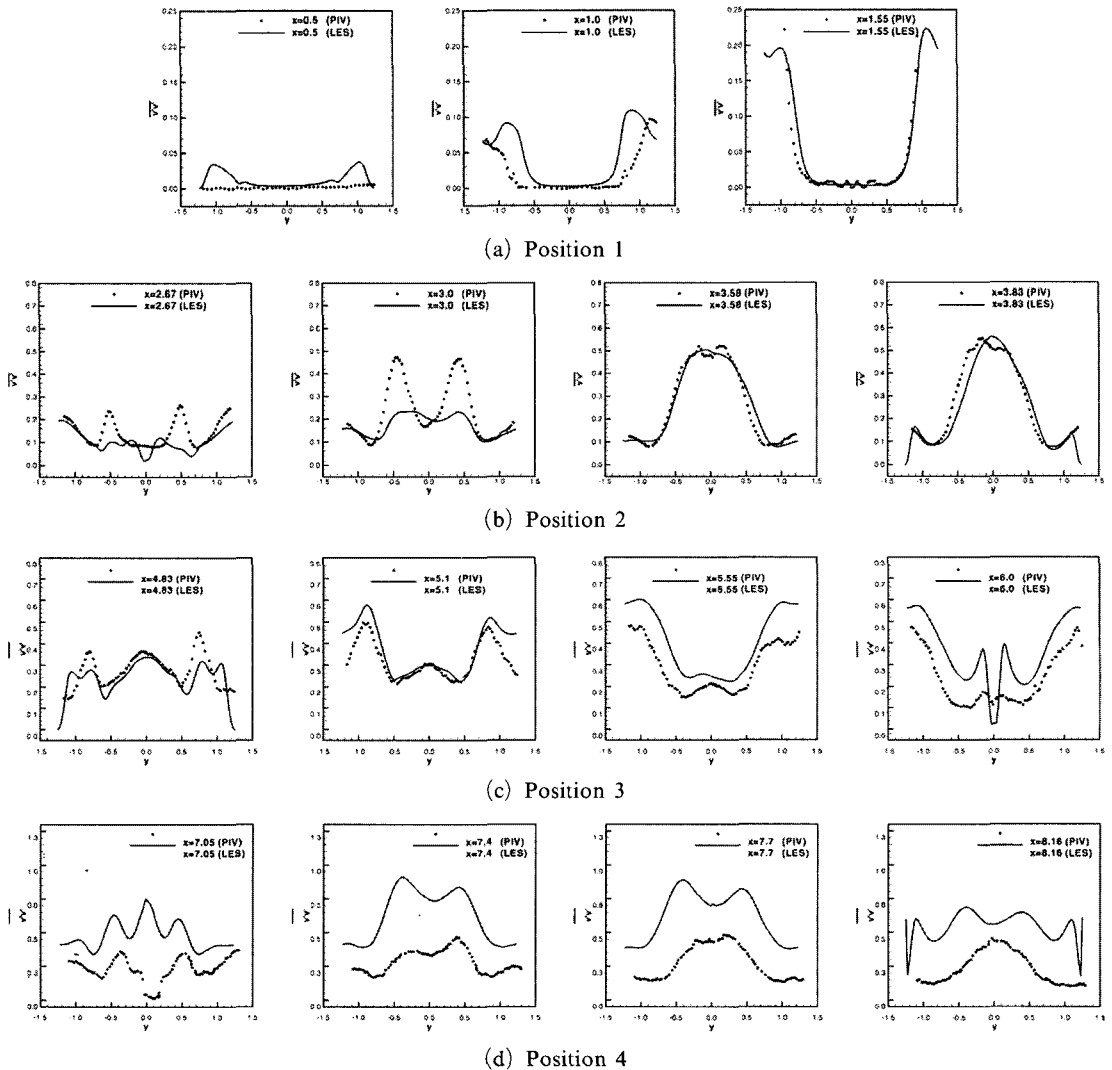
Fig. 9 Comparison of the time-averaged cross-streamwise turbulence intensity obtained from the present calculation with PIV experiment : (-) this study, (•) PIV experiment
