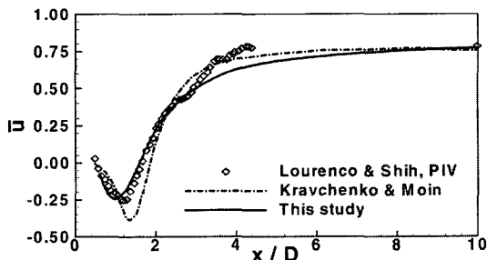
Fig. 3 Comparison of time-averaged streamwise velocity along the centerline for the flow past a single cylinder with PIV and DNS data
