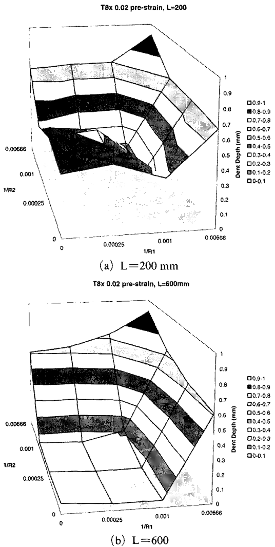
Fig. 14 Predicted dynamic dent depths for unequally double curved 6111 T8X, 2% pre-strain panels
