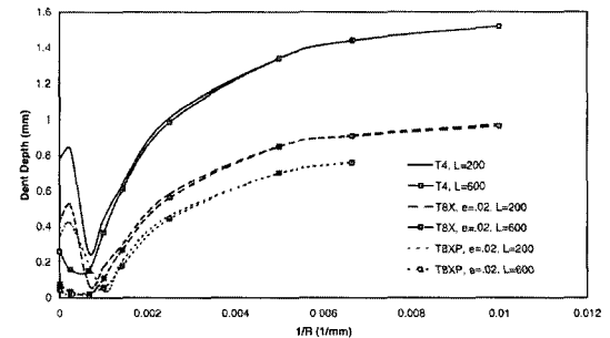
Fig. 10 Dynamic dent depths predicted for the 6111 T8x, 2% pre-strain panels. Impact velocity= 4.89 m/s
