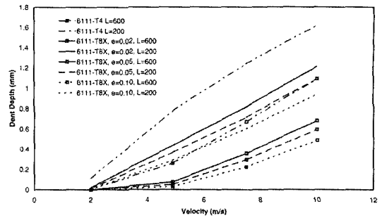
Fig. 13 Dynamic dent depth as a function of impact velocity for 1 mm flat panels comparing various material conditions (heat treatment and pre-strain)
