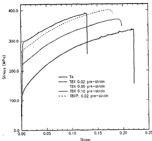
Fig. 4 Stress-strain curves adopted for the sheet materials
