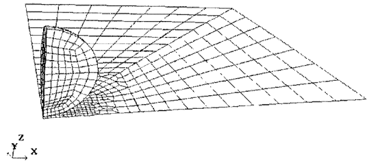
Fig. 2 Finite element mesh used for the R4000 × R4000, 200 mm panel
