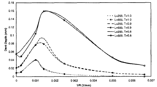
Fig. 9 Static dent depths predicted for the 6111 T8x, 2% pre-strain panels. Maximum load=155 N
