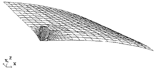
Fig. 3 Finite element mesh used for the R1500 × R1000, 600 mm panel
