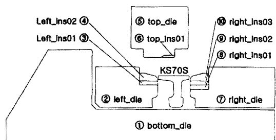
Fig. 2 Schematic illustration of forging dies
