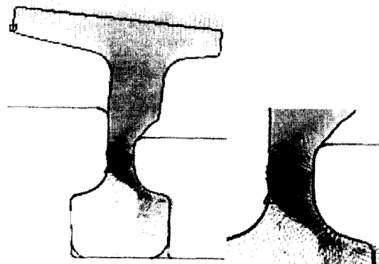
(b) Result of the simulation
