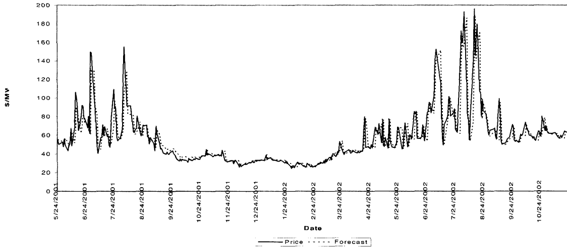
Fig. 1 Actual Versus Forecast Day-Ahead New York City Electricity Prices (May 24, 2001 Through November 22, 2002) Using GARCH, Omitting Extreme Values
