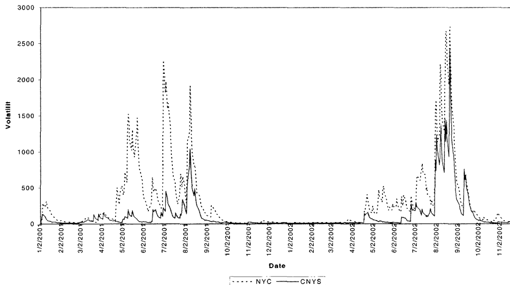
Fig. 3 Comparison of the Volatility of the Electricity Prices in New York City and Central New York State for the Period of January 1, 2001 to November 22, 2002)
