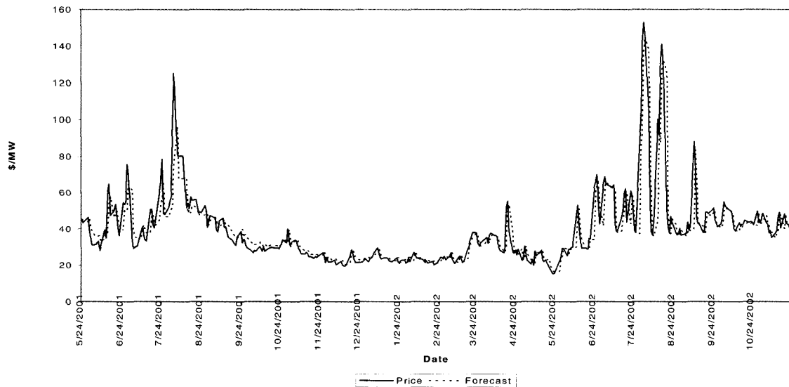
Fig. 2 Actual Versus Forecast Day-Ahead Central New York State Electricity Prices (May 24, 2001 Through November 22, 2002) Using GARCH, Omitting Extreme Values
