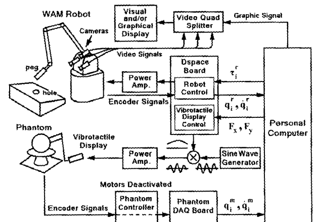
Fig. 4. Block diagram representation of the experimental setup.
