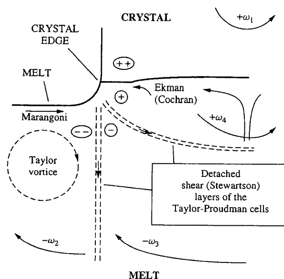
Fig. 13. More than six types of flow, differing in direction and/or velocity, below the edge of a Czochralski-grown crystal for the case of crystal rotation +\omega_1 and crucible counterrotation -\omega_2 above the critical Rossby number, after Scheel and Sielawa [69].
