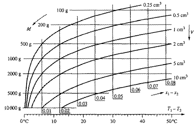
Fig. 6. Nomogram to read the experimental parameters for growth of KTN solid solution crystals of a specified maximum inhomogeneity x_1 - x_2 and volume v . M = mass of the melt, T_1 - T_2 is the cooling interval (Rytz and Scheel [35]).
