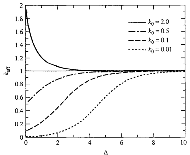
Fig. 8. The effective distribution coefficient as a function of the exponent (v\delta/D) = \Delta from the Burton-Prim-Slichter equation (4) for four values of k_0 , from Scheel and Swendsen [29].
