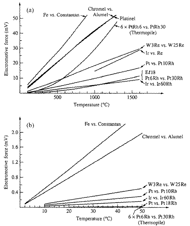
Fig. 11. The electromotive forces of various common thermocouples a) for high temperatures, b) for the temperature range 0° to 50°C. Note that the thermopile of 6 x PtRh6% versus PtRh30% has a very high sensitivity at high temperatures and practically no sensitivity around room temperature (Scheel and West [46], from Elwell and Scheel [33]).
