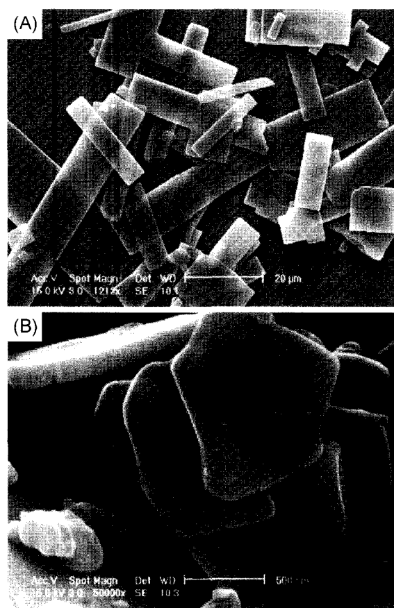
Fig. 1. SEM micrographs of (A) (\text{C}_6\text{H}_5\text{CH}_2\text{NH}_3)_2\text{CuCl}_4 and (B) (\text{NH}_3\text{C}_6\text{H}_4\text{C}_2\text{H}_4\text{C}_6\text{H}_4\text{NH}_3)\text{CuCl}_4 .
