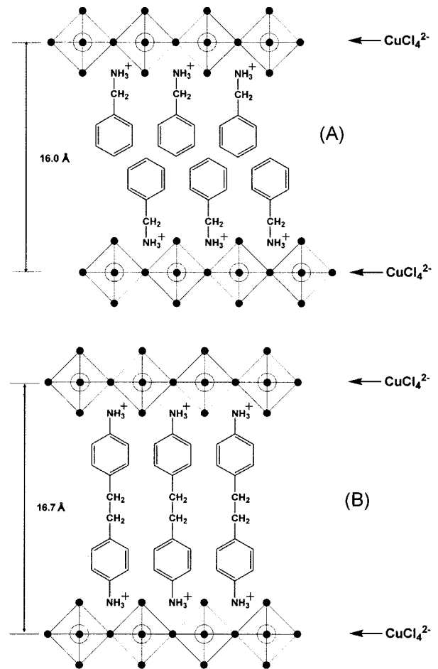
Fig. 3. Schematic illustration for the orientation of (A) (\text{C}_6\text{H}_5\text{CH}_2\text{NH}_3)_2\text{CuCl}_4 and (B) (\text{NH}_3\text{C}_6\text{H}_4\text{C}_2\text{H}_4\text{C}_6\text{H}_4\text{NH}_3)\text{CuCl}_4 .
