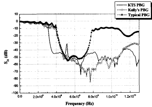
(c) Kelly의 PBG와 KTS PBG의 주파수특성 (c) Frequency Characteristic of Kelly's PBG and KTS's PBG
