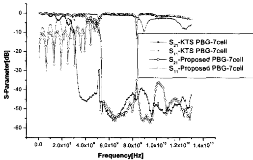
(b) 제안된 PBG구조의 주파수특성 (b) Frequency response of the proposed PBG structure
