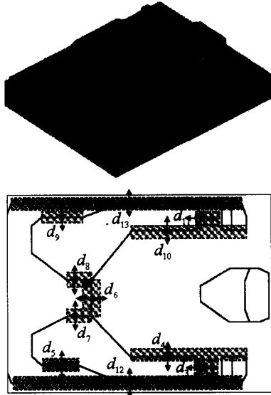
Fig. 6 Slider model
