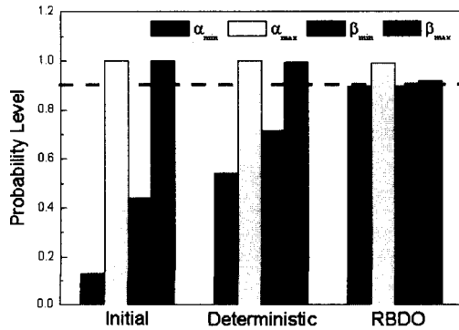
Fig. 7 Probability of the RBDO
