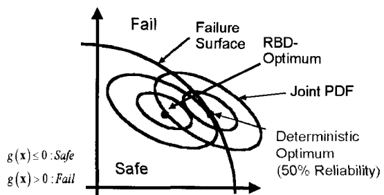
Fig. 3 Reliability-based design optimization
