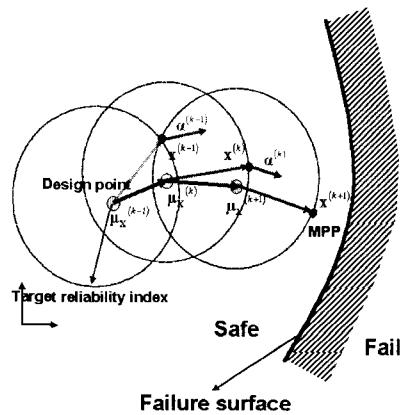
Fig. 5 SLSV concept
