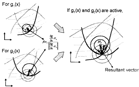
Fig. 4 Moving initially inactive design
