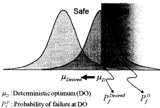
Fig. 2 Design considering uncertainty
