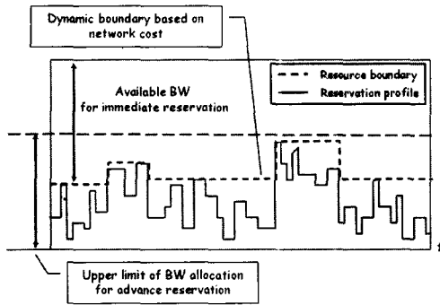
Figure 7. Resource sharing with dynamic resource boundary.
