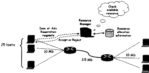
Figure 10. Simulation topology.
