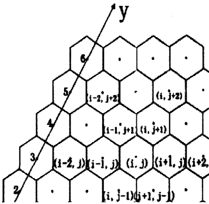
Fig 2. Cell mapping
