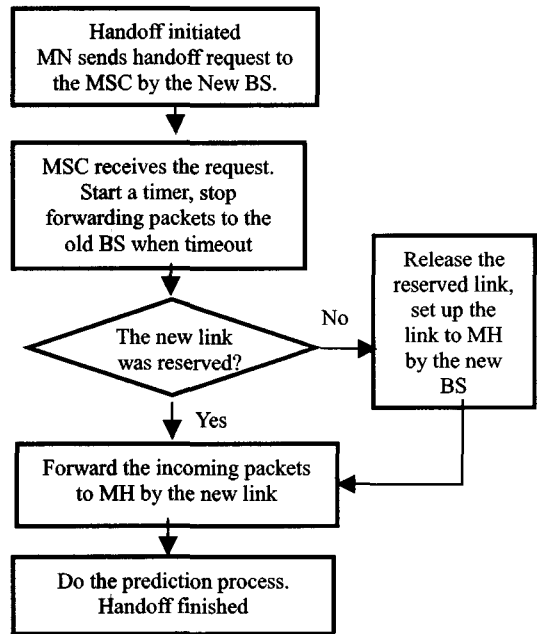
Fig 3. The handoff procedure
