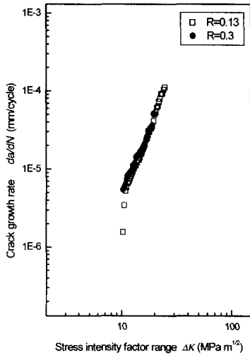
Fig. 6 Relation between stress intensity factor range and crack growth rate
