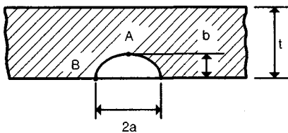
Fig. 13 Geometry of stress intensity factor under bending loads
