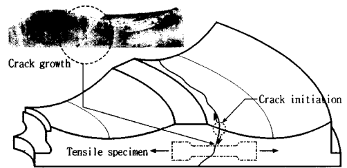
Fig. 2 Sampling direction of tensile and bending specimen and fracture process of table liner
