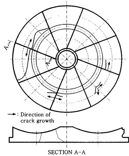
Fig. 1 Fracture aspect of table liner for vertical roller mill
