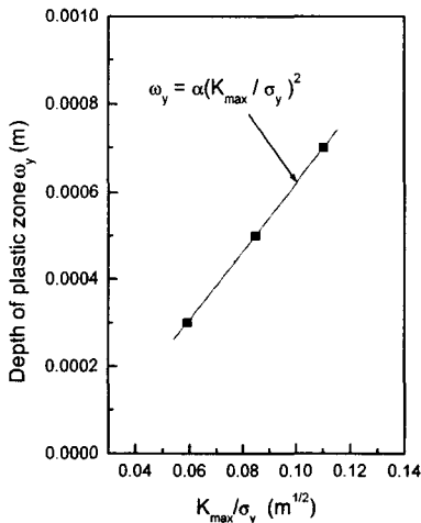
Fig. 11 Relationship between plastic zone depth and maximum stress intensity factor to yield strength
