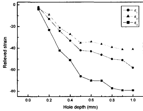
(b) K_{\max} = 20.47 \text{ MPa m}^{1/2}
