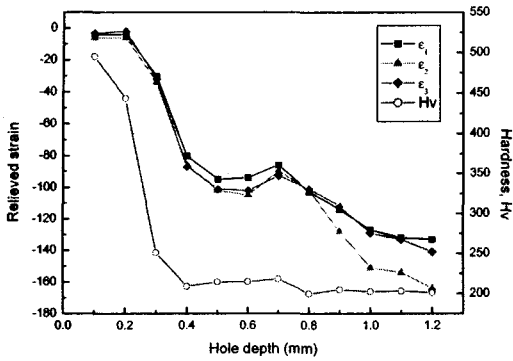
Fig. 9 Comparison between relieved strain and microhardness for shot-peening
