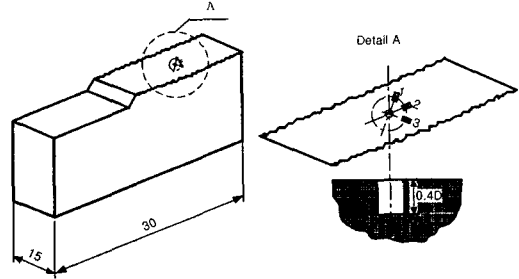
Fig. 4 Schematic illustration of HDM on fatigue fractured surface of SEB
