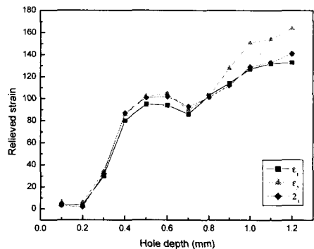
Fig. 8 Relieved strain plotted against the depth from fatigue fractured surface for shot-peening
