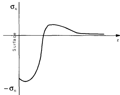
Fig. 7 Typical residual stress of shot-peening
