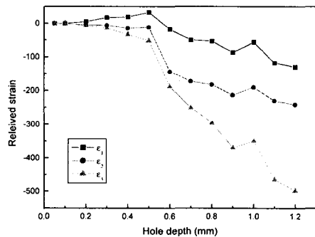
Fig. 12 Relieved strain plotted against the depth from fatigue fractured surface for table liner
