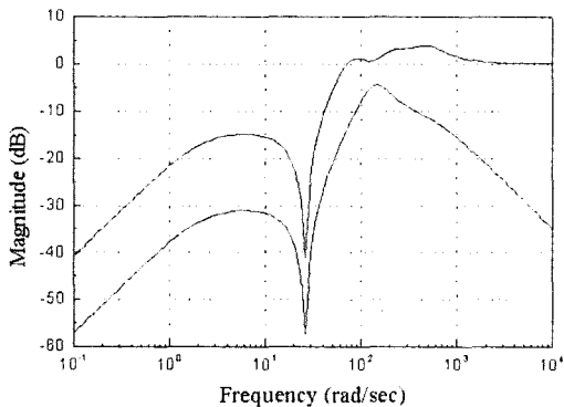
Fig. 5 Singular value diagram of the closed-loop transfer function matrix from disturbances to outputs
