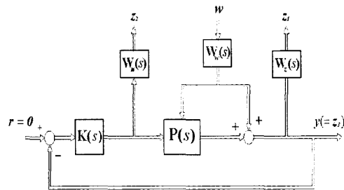
Fig. 3 Feedback control system for the generalized plant with weighting functions
