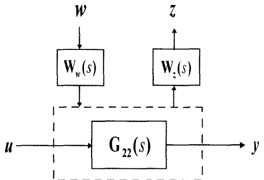
Fig. 4 Weightings having poles on the j\omega axis
