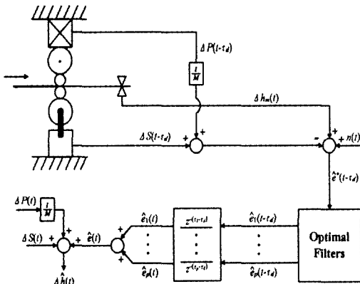
Fig. 2 Eccentricity estimator and output thickness prediction
