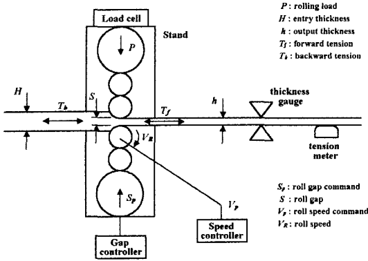
Fig. 1 Rolling process of a mill stand
